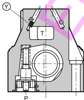
pilot always internal Y: plug M6x8 for external drain
